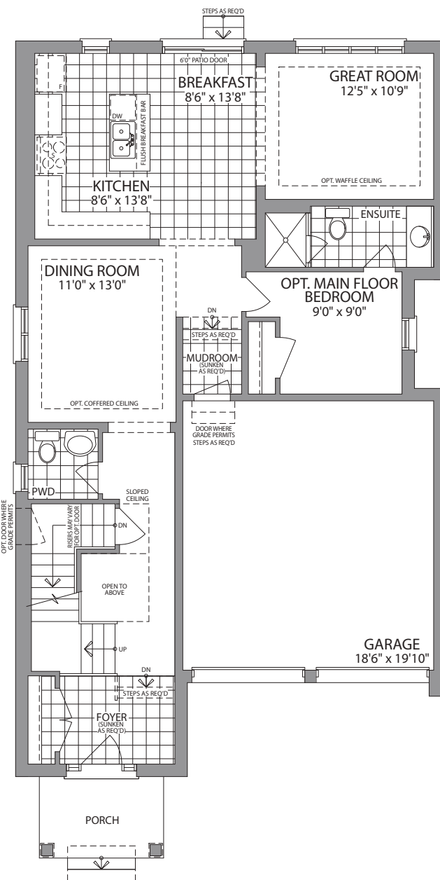
GROUND FLOOR W/OPT. BEDROOM ELEVATION A
