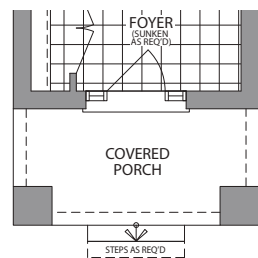
GROUND FLOOR W/OPT. BEDROOM ELEVATION B
