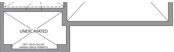
BASEMENT ELEVATION B
