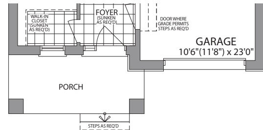
GROUND FLOOR ELEVATION C
