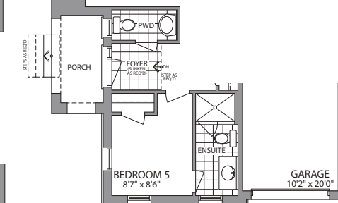
OPT. GROUND FLOOR W/5 BEDROOMS ELEVATION B
