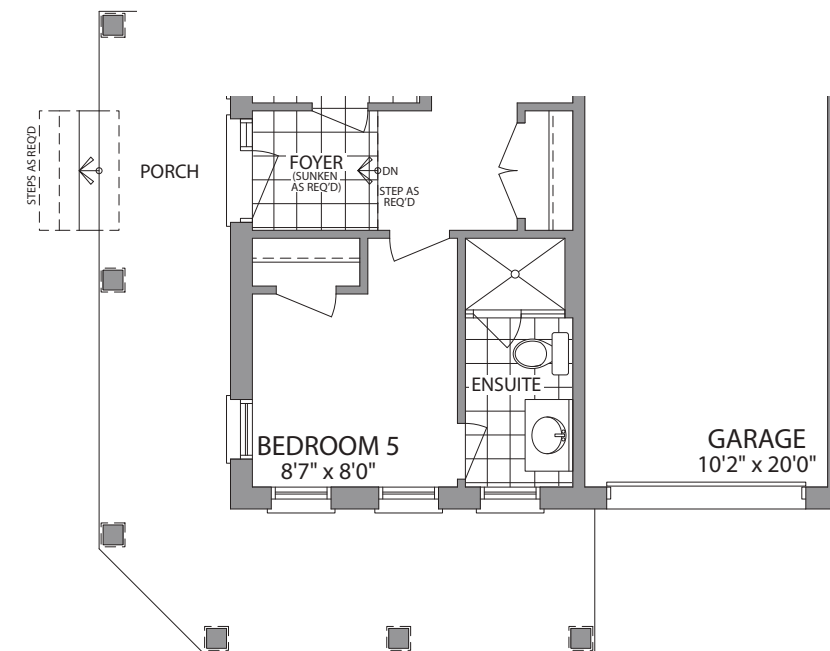
GROUND FLOOR W/OPT. BEDROOM ELEVATION A
