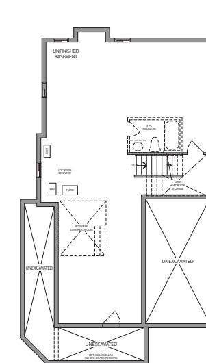
BASEMENT ELEVATION A
