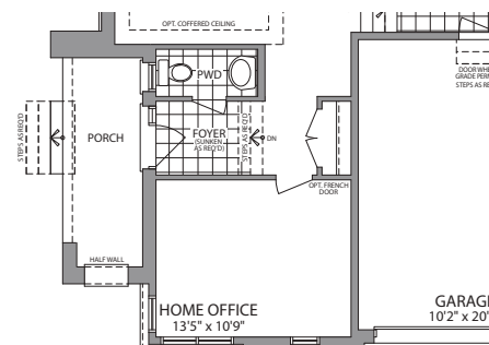
GROUND FLOOR ELEVATION C
