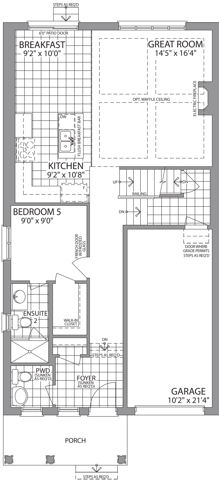
OPT. GROUND FLOOR W/5 BEDROOMS ELEVATION A
