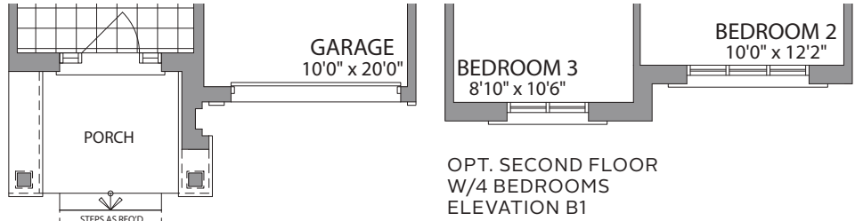
GROUND FLOOR ELEVATION B1
