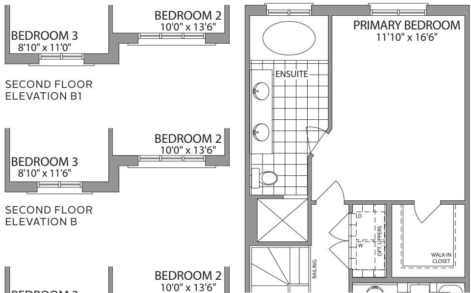
OPT. SECOND FLOOR W/2 PIECE LAUNDRY ELEVATION A, A1, B & B1
