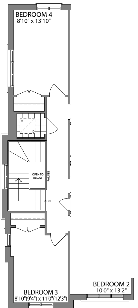
OPT. SECOND FLOOR W/4 BEDROOMS ELEVATION B
